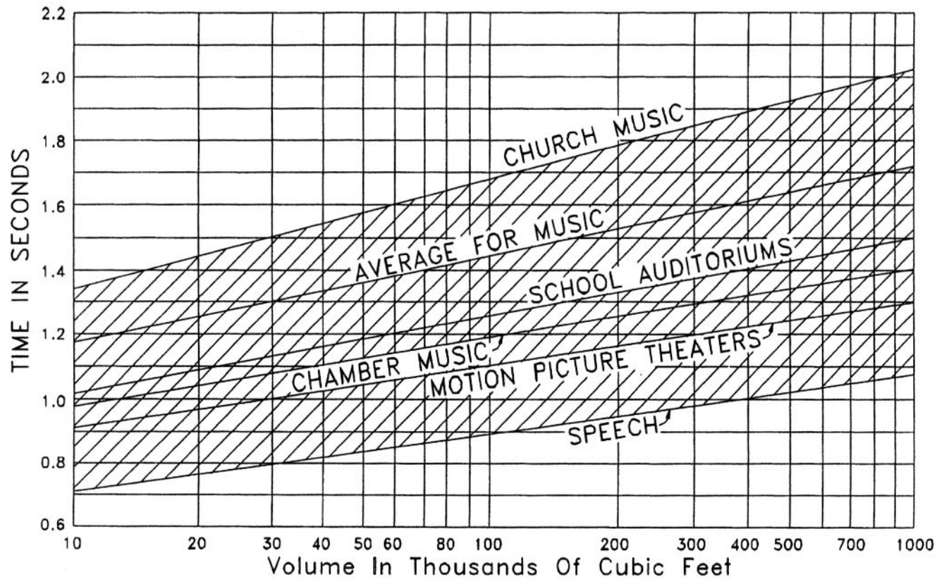
Recommended Optimum Reverberation Times For Various Room Uses. (Reproduced with permission from Acoustical Designing in Architecture, V.O. Knudsen and C.M. Harris, America Institute of Physics, Paperback Edition, 1980. Copyright 1950, 1978, Acoustical Society of America.)
